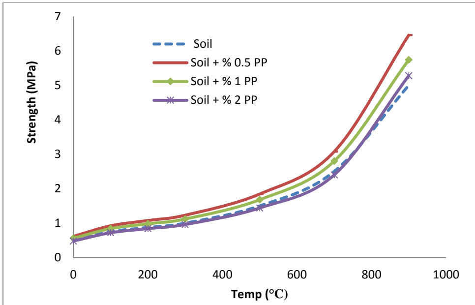
Figure 8. Effect of heat on soil unconfined compressive strength with PP
