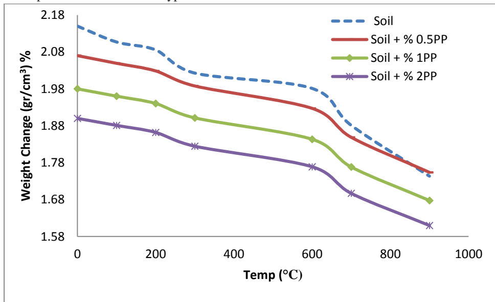
Figure 5. Weight changes of soil samples subjected to heat in PP fibers
