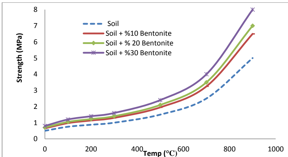
Figure 10. Effect of heat on soil unconfined compressive strength with bentonite
