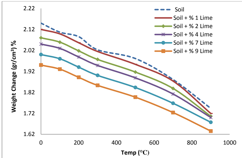
Figure 6. Weight changes of soil samples subjected to heat for samples containing lime
