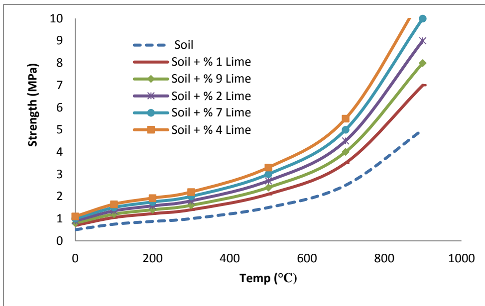
Figure 9. Effect of heat on soil unconfined compressive strength with lime
