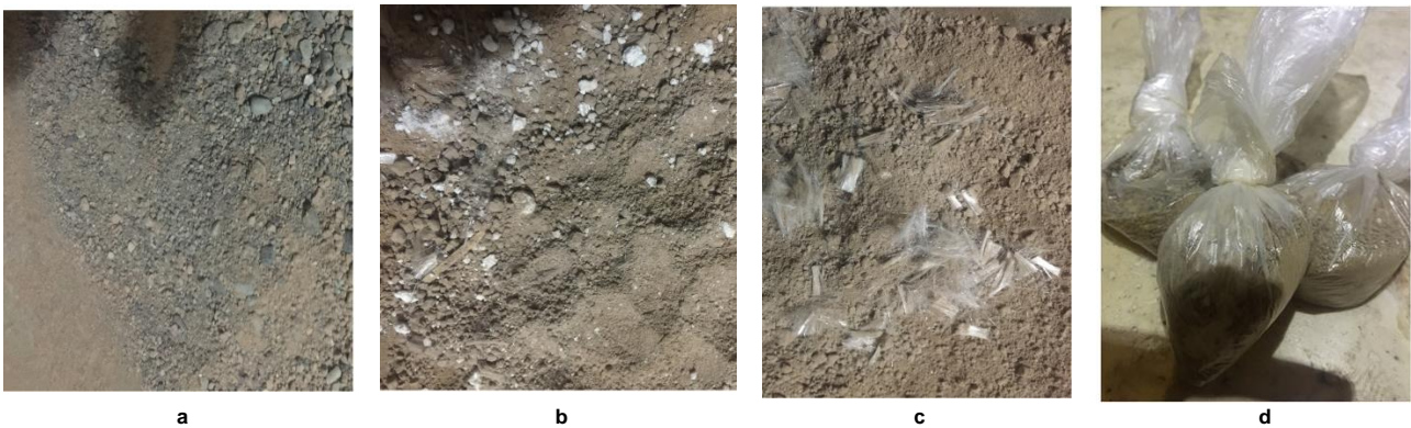
Figure 3: Stabilization of soil with a) bentonite, b) lime, c) polypropylene; d) prepared samples
