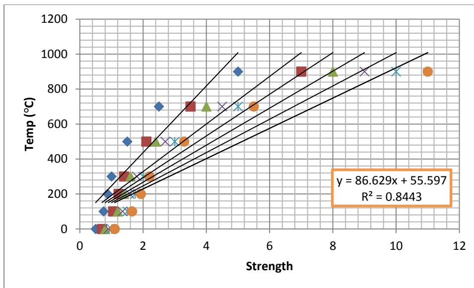
Figure 11. Relationship between unconfined compressive strength and heat
