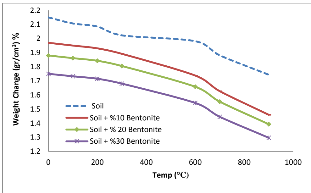
Figure 7. Weight changes of soil samples subjected to heat for samples containing bentonite
